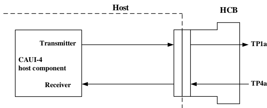
Figure 4: IEEE 802.3 CAUI-4 compliance points TP1a, TP4a
