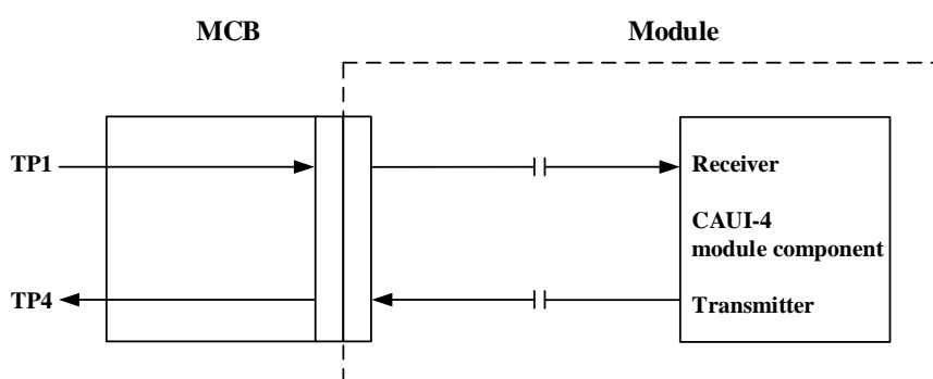
Figure 5: IEEE 802.3 CAUI-4 compliance points TP1, TP4
